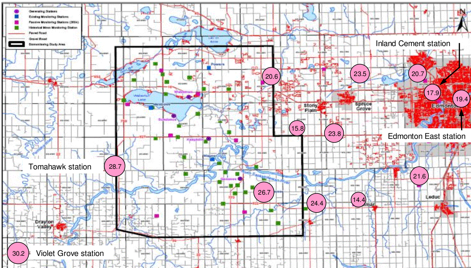
Figure 3. Bubble plot of annual average O 3 concentrations at passive monitoring locations and at selected continuous monitoring station locations in central Alberta during 2005.
